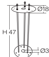
code 00A405.01P Anchor Bolt
